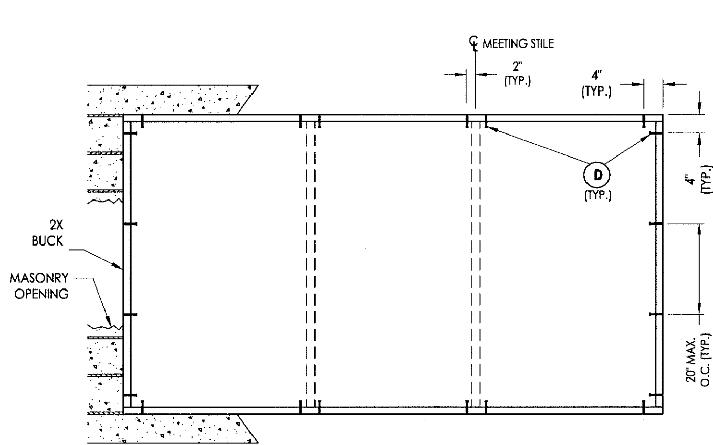
BUCK ANCHORING
