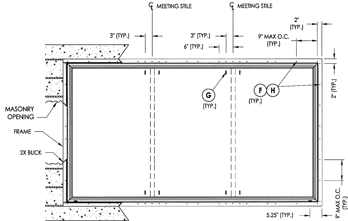
FRAME ANCHORING
