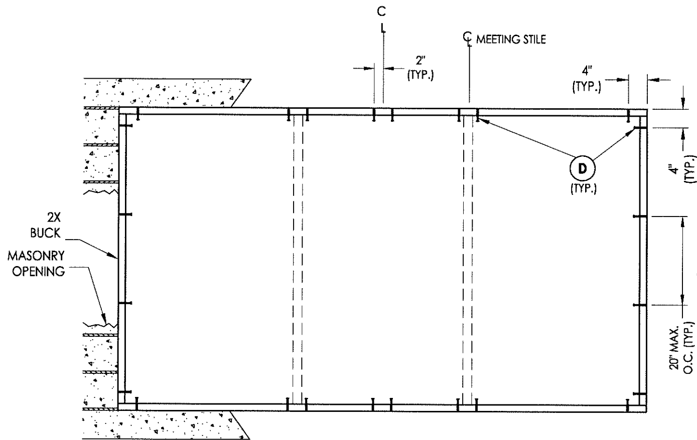
BUCK ANCHORING
