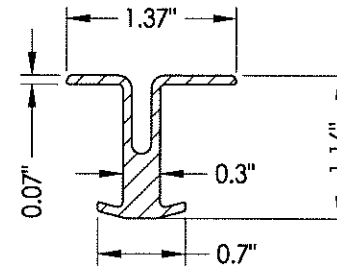
12 HEAD TRACK 6\"/>
