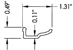
28 GLAZING BEAD
