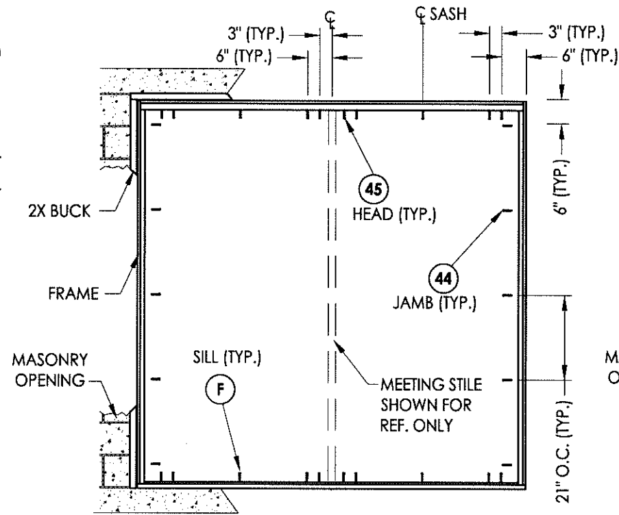
FRAME ANCHORING 2X
