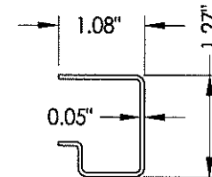
53 REINFORCEMENT Stile
