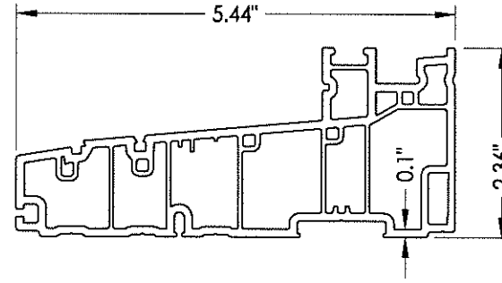
12 FRAME SILL
