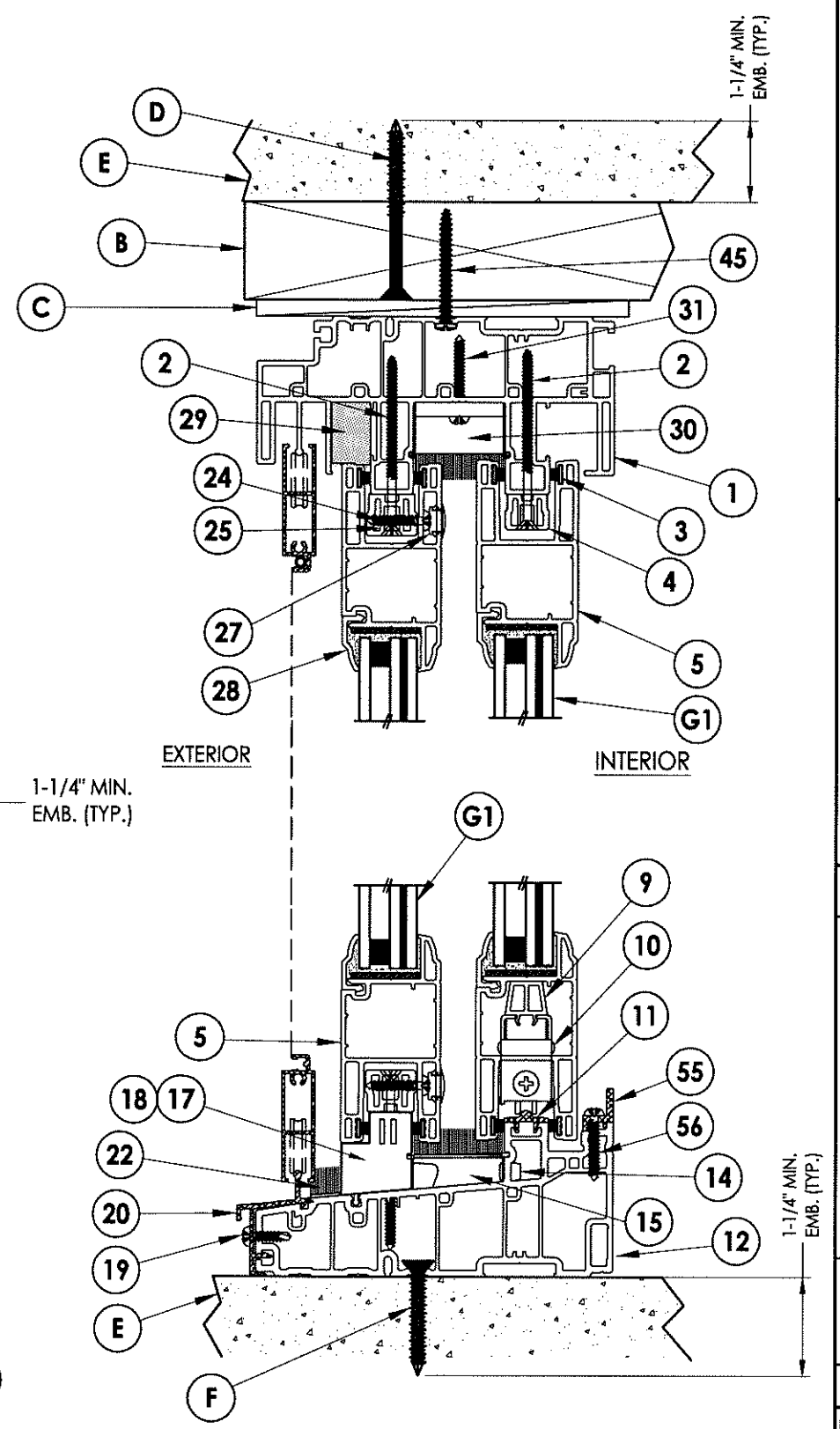
3 VERTICAL CROSS SECTION 2 Shown w/ 2X Buck at head & Direct to Masonry @ sill
