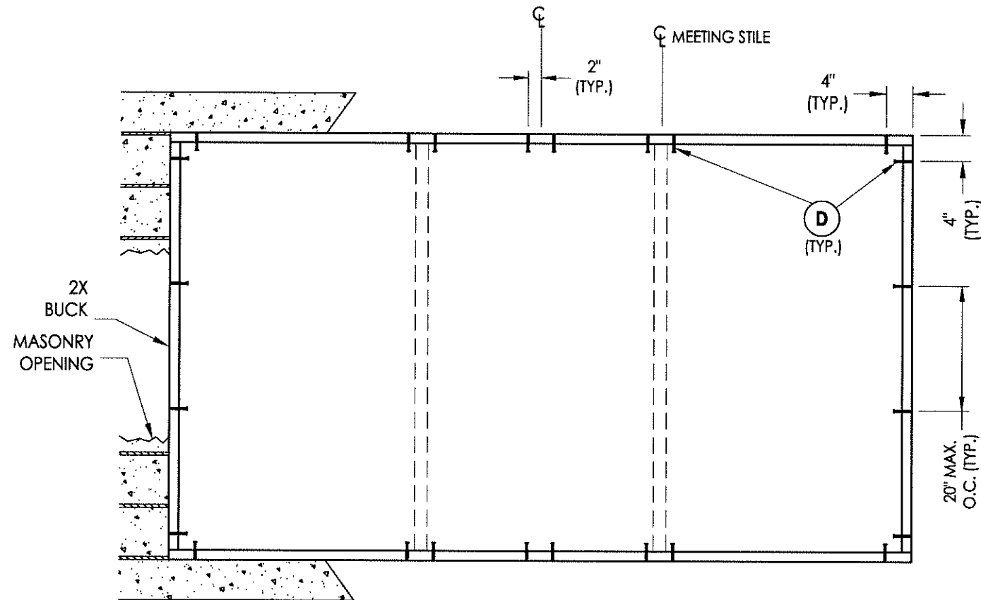
BUCK ANCHORING
