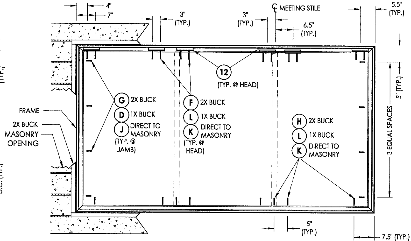
FRAME ANCHORING
