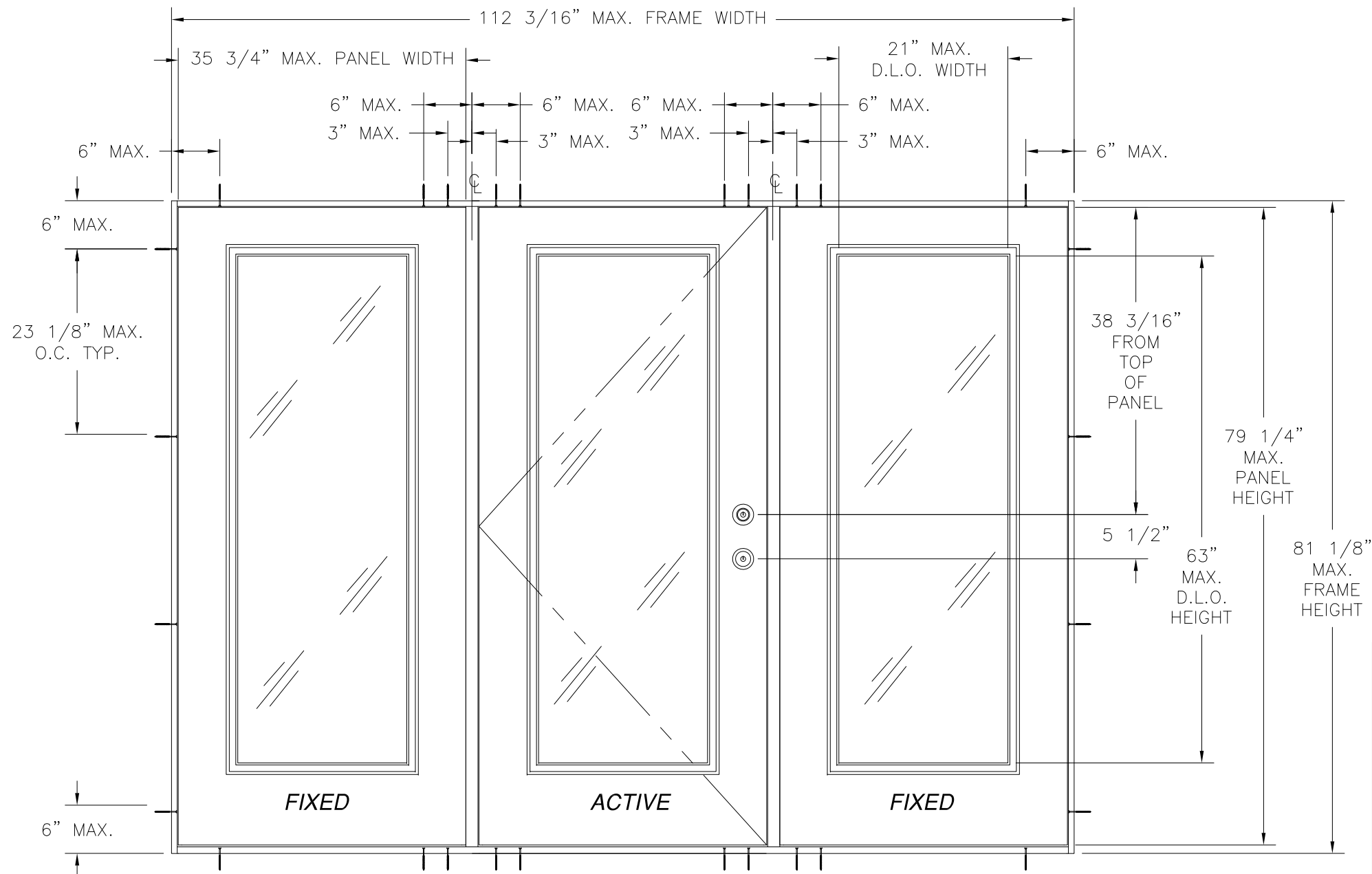
PLASTPRO INSERT GLAZED FIBERGLASS 6'8 OS OXO DOOR EXTERIOR VIEW
