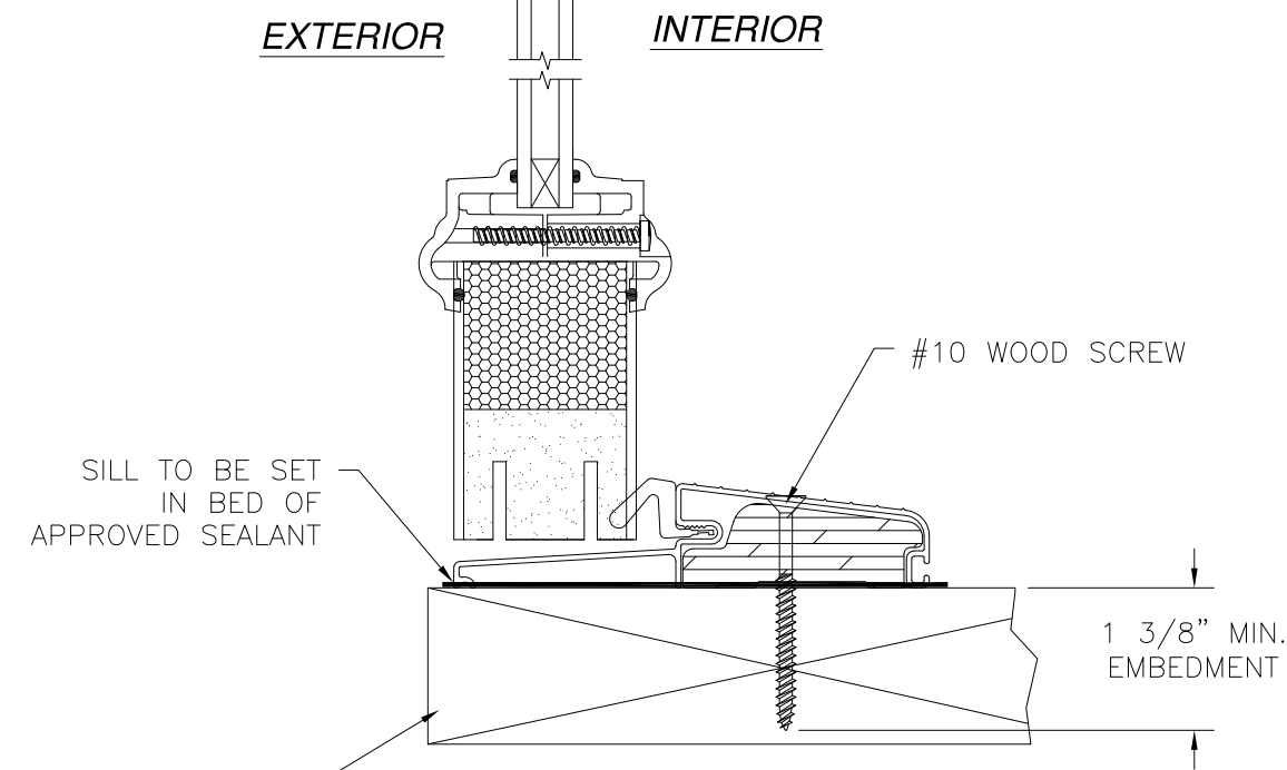
VERTICAL CROSS SECTION 2X BUCK/WOOD FRAMING DOOR SHOW, SIDELITE SIMILAR
