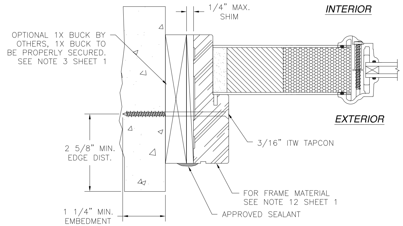
HORIZONTAL CROSS SECTION MASONRY/CONCRETE INSTALLATION SIDELITE JAMB SHOWN, STRIKE AND HINGE JAMB SIMILAR
