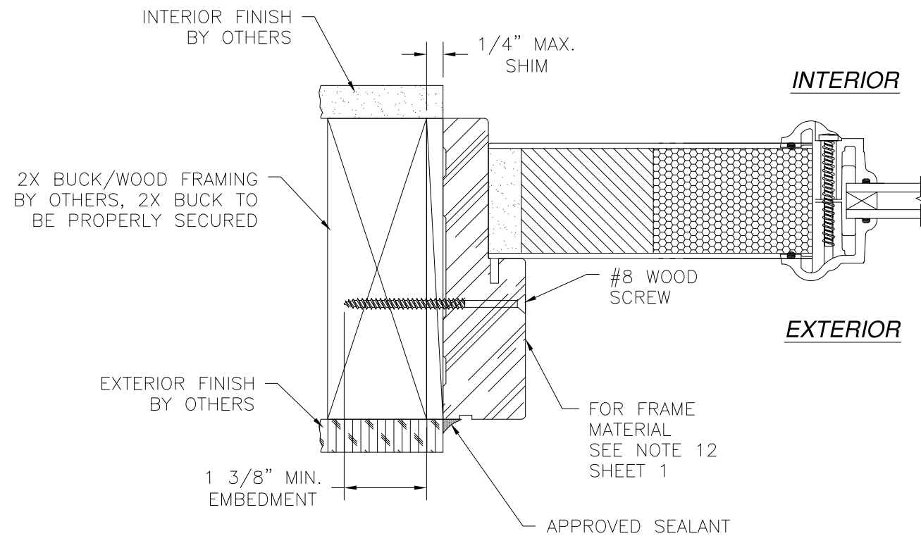
HORIZONTAL CROSS SECTION 2X BUCK/WOOD FRAMING SIDELITE JAMB SHOWN, STRIKE AND HINGE JAMB SIMILAR
