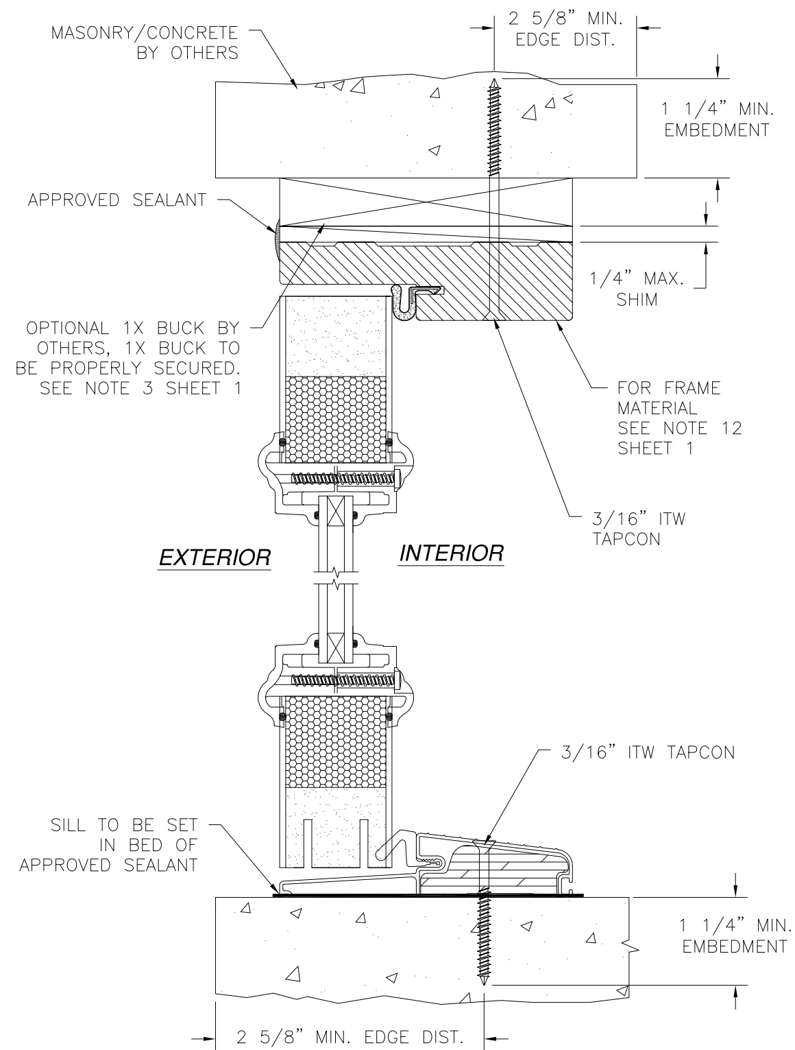
VERTICAL CROSS SECTION 2X BUCK/WOOD FRAMING DOOR SHOWN, SIDELITE SIMILAR
